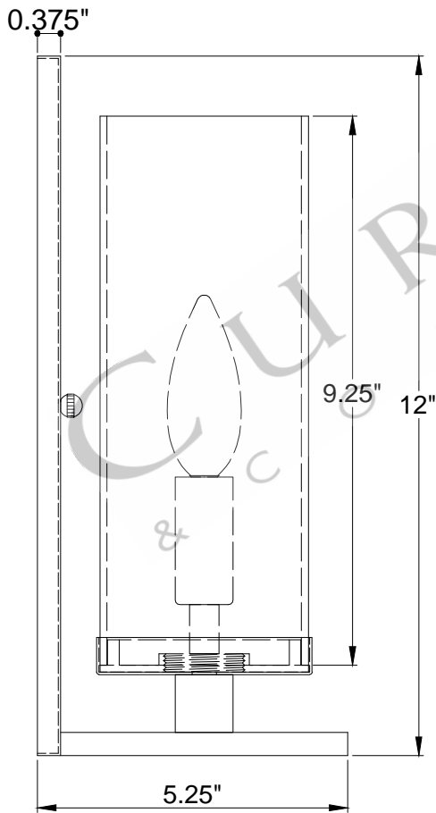
SIDE VIEW
